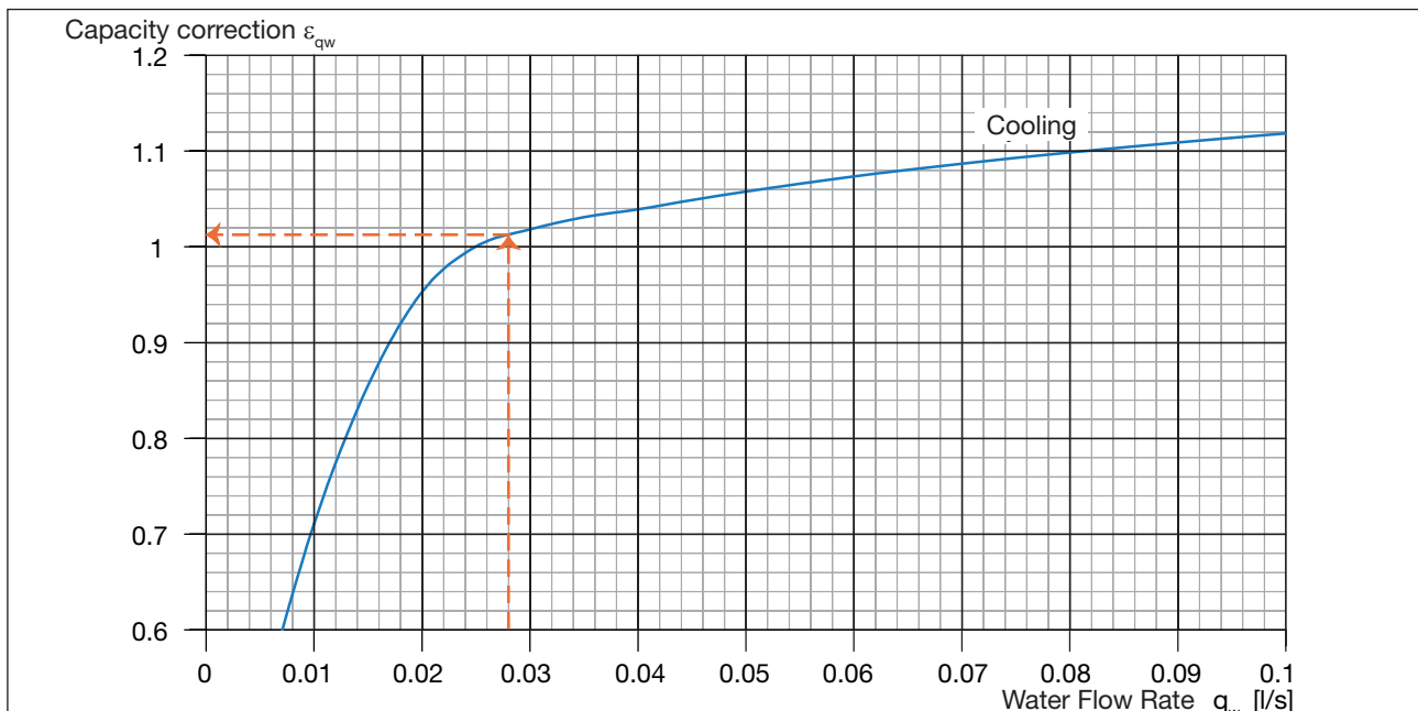
Diagram 2. Capacity correction \epsilon_{qw} for water flow for cooling average water temperature = 15°C.
