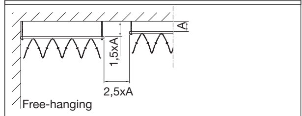
Figure 2-4. Installation dimensions for Carat.
