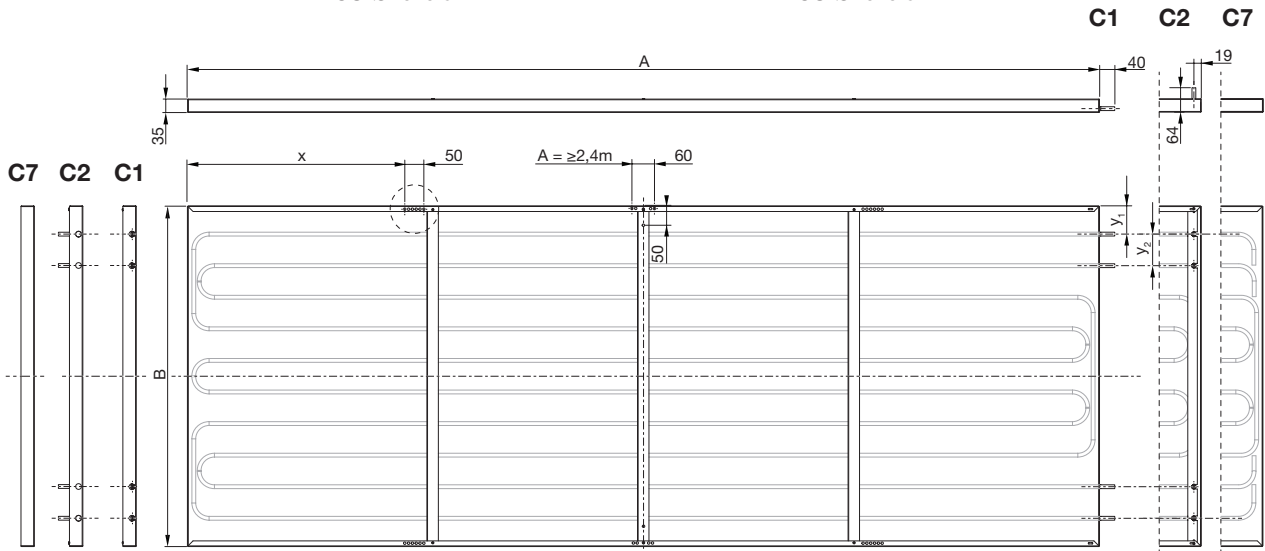
Dimensions of heating and cooling panel
