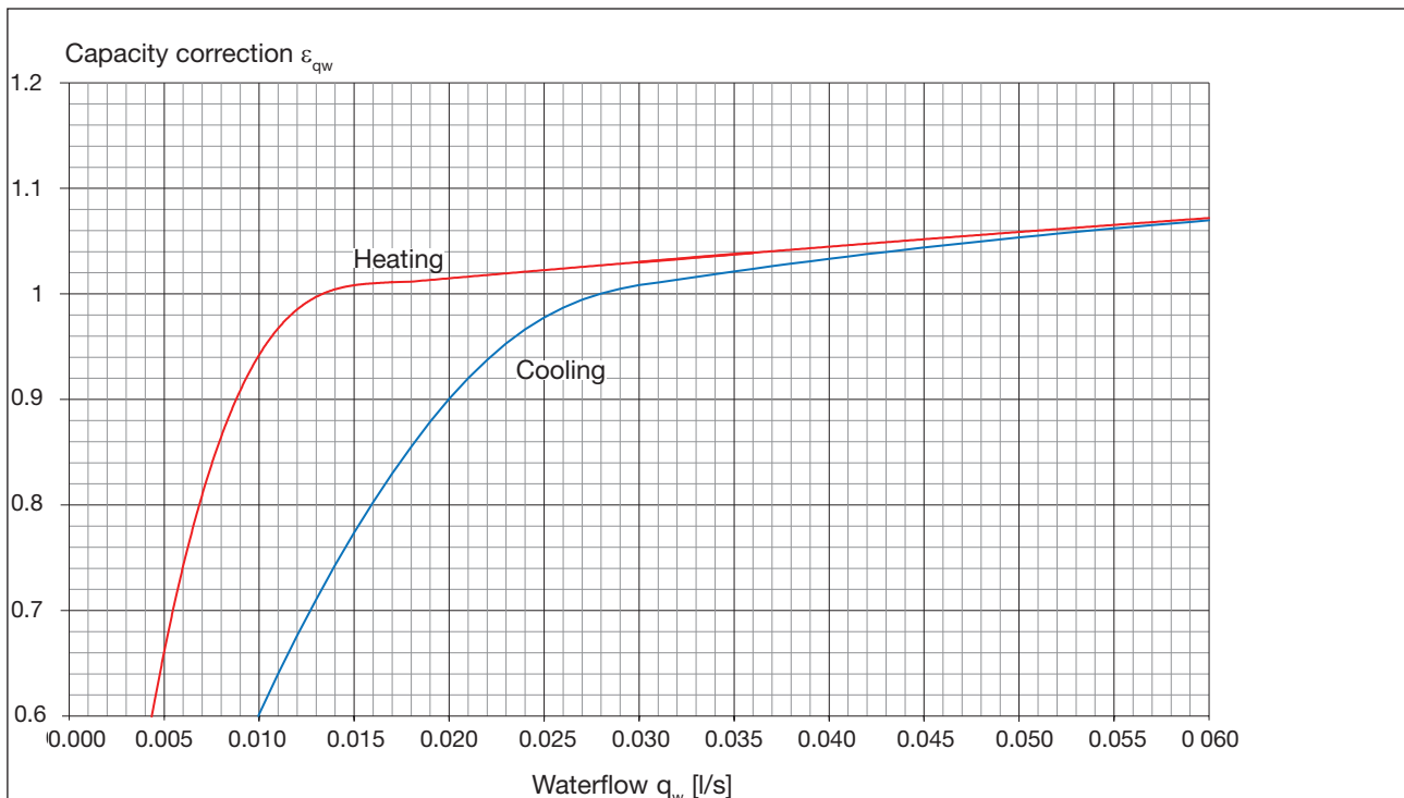
Diagram 3. Capacity correction \epsilon_{q_w} as a function of waterflow q_w .
