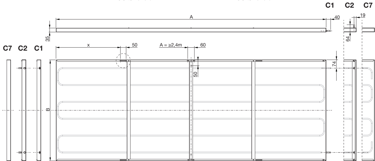
Dimensions of heating or cooling panel
